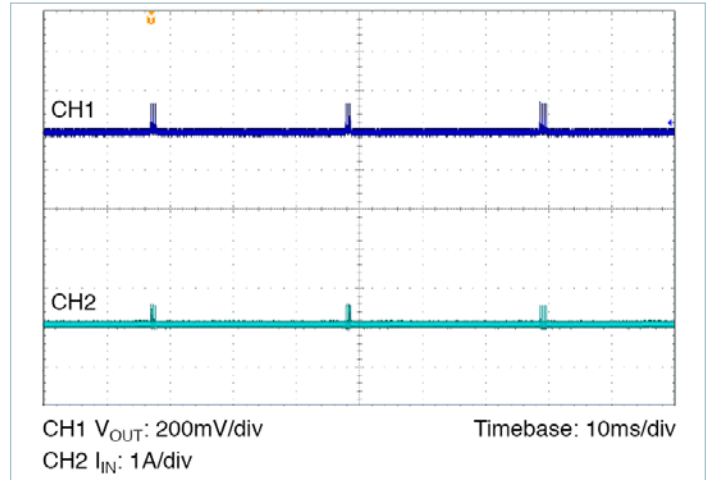
Figure 80 — Output Short Circuit, Nominal Line
