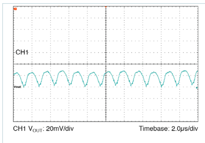
Figure 52 — Output Voltage Ripple: Nominal Line, Nominal Trim, 50% load, C OUT = 12 x 47µF Ceramic
