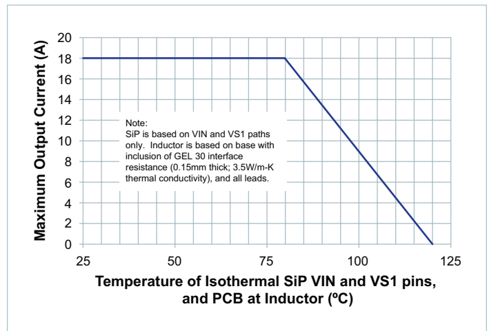
Figure 82 — System Thermal Specified Operating Area: Max I OUT at Nominal Trim vs. temperature at locations noted
