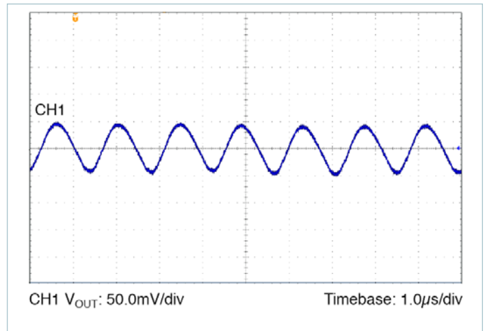
Figure 81 — Output Voltage Ripple: Nominal Line, Nominal Trim, 50% load, C OUT = 8 x 10µF Ceramic
